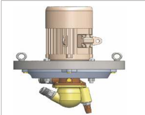
Nuclear Active Waste Water Transfer- Nuclear Submarine Project, Defence Machinery Design Establishment, India
